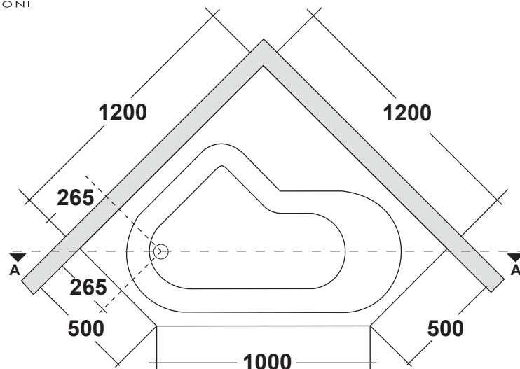
Vista in pianta plan view
